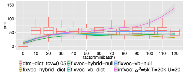
(b) 20 newsgroups , S = 155 , K = 50 , \kappa = 0.8 and \tau_0 = 64
