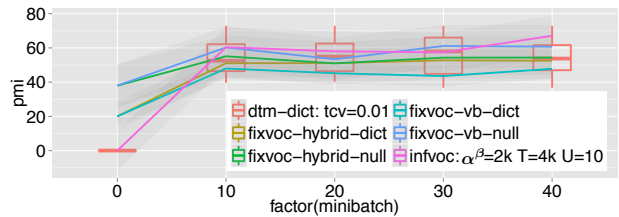
(a) de-news , S = 245 , K = 10 , \kappa = 0.6 and \tau_0 = 64
